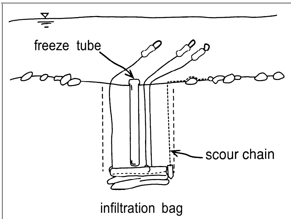
Figure 5-Integrated setup for measuring volume of infiltrated sediment (infiltration bag), depth of deposition of fine sediment (freeze tube), and depth of scour and fill (scour chain).
