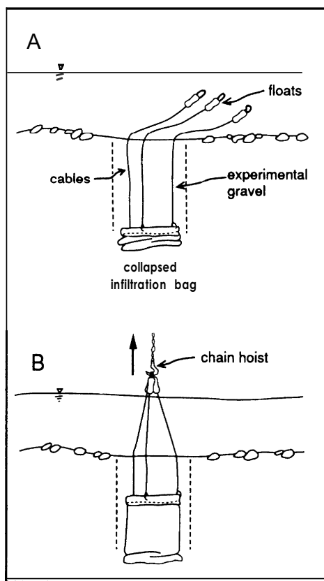
Figure 4-Installation (A) and recovery (B) of an infiltration bag.
