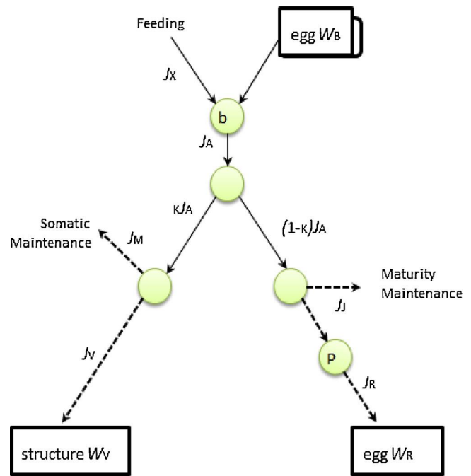
Fig. 1. The Schematic description of DEBkiss model. Arrows indicate energy fluxes ( \rightarrow assimilated and mobilized energies, -\rightarrow allocated energy) that drive the dynamics of the state variables, depicted in boxes (Structure, W_V and Reproductive Buffer, W_R ). Energy enters the animal as food, J_x , and then assimilated at a rate J_A . The assimilated food will be mobilized in proportion of k to somatic maintenance and structure) and 1 - k to maturity and reproduction. The kJ_A proportion of mobilized flux will be allocated to somatic maintenance, J_M and growth J_V . The (1-k)J_A flux divided as maturity maintenance flux J_J and reproduction flux, J_R .
