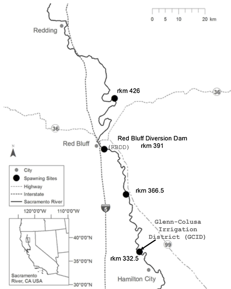
Fig. 2. Location map of the area considered in the simulation model (Table 3). The four known spawning and hatching locations of the green sturgeon are shown as black circles.
