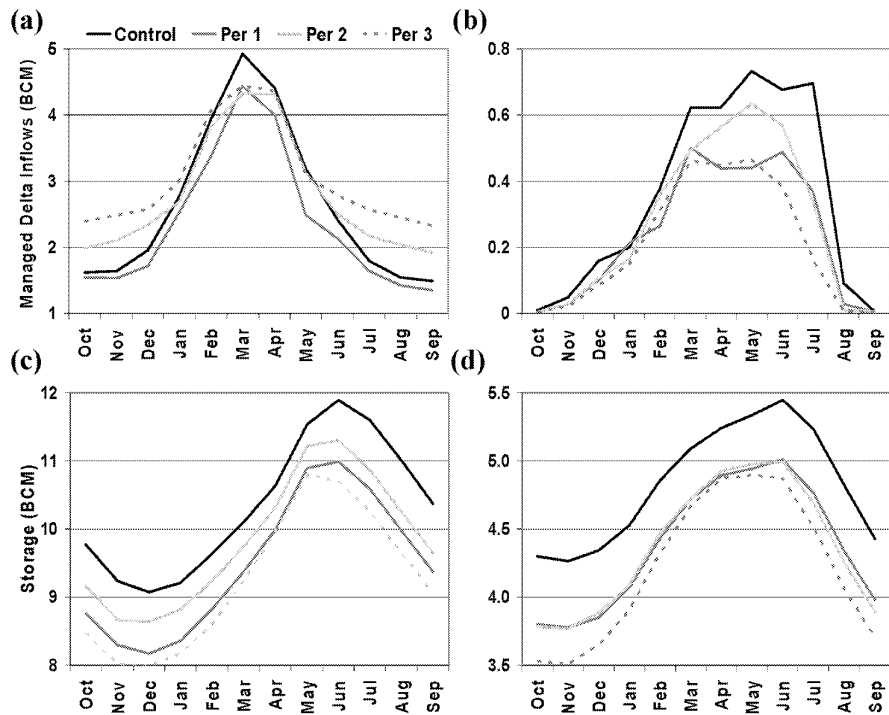
Figure 6. Predicted 2000–2008 mean monthly regulated Delta inflows and Sacramento and San Joaquin total storages given current operating rules and year 2001 demands and hydrologic development: (a) Regulated flows at the mouth of the Sacramento River and (b) at the mouth of the San Joaquin River; (c) total reservoir storage north of the Delta (i.e., Sacramento River System) and (d) south of the Delta (i.e., San Joaquin River System).
