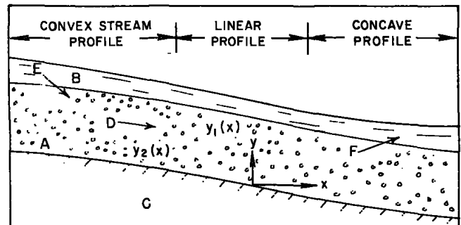
FIGURE 2.—Description of terms and properties relating to waterflow within a streambed. A, porous bed; B, ambient stream; C, impermeable stratum; D, intragravel flow; E, downwelling; F, upwelling; y_1, bed surface profile; y_2, impermeable stratum profile.
