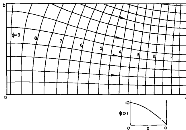
FIGURE 6.—Flow net for convex parabolic surface potential.
