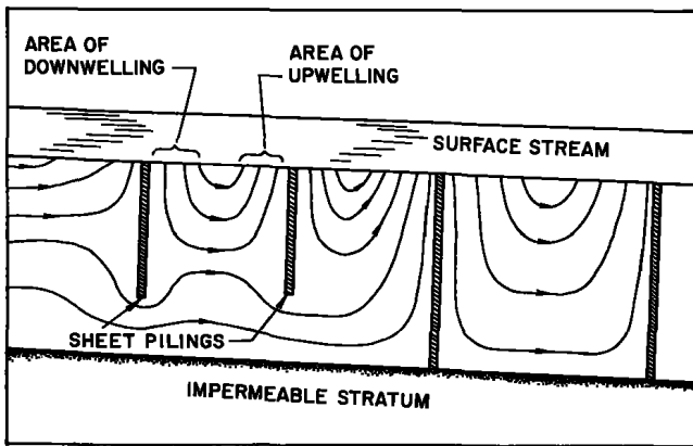
FIGURE 13.—Interchange induced by sheet pilings.
