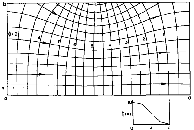
FIGURE 8.—Flow net for sigmoid surface potential.
