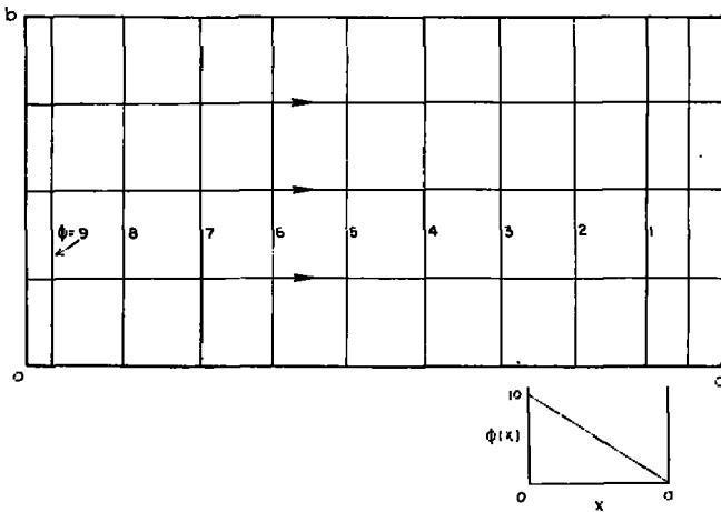
FIGURE 5.—Flow net for straight-line-surface potential b/a = 1/2 .
