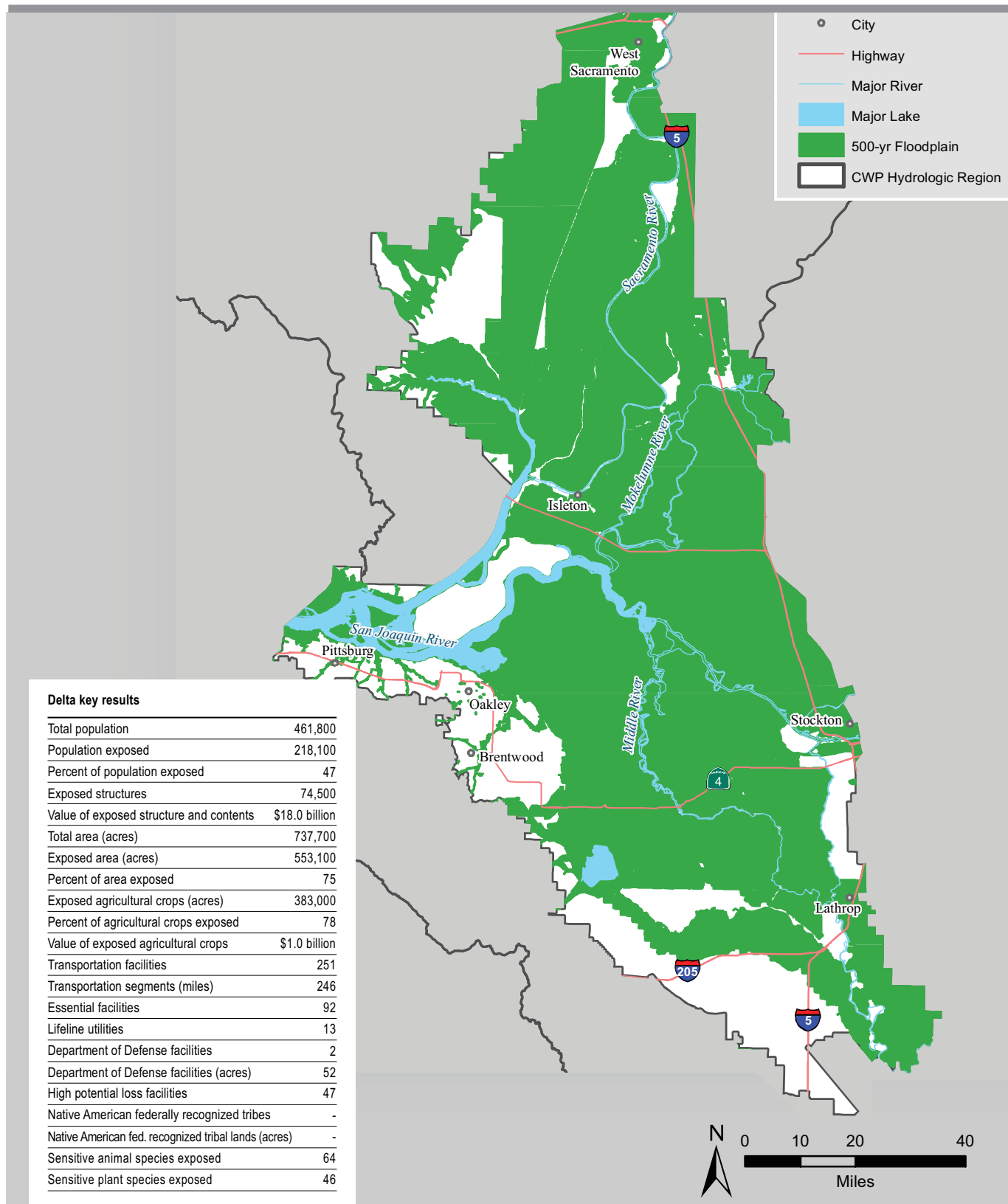
Figure D-11 Statewide Flood Hazard Exposure Summary for the Sacramento-San Joaquin Delta Region 500-year Floodplain
