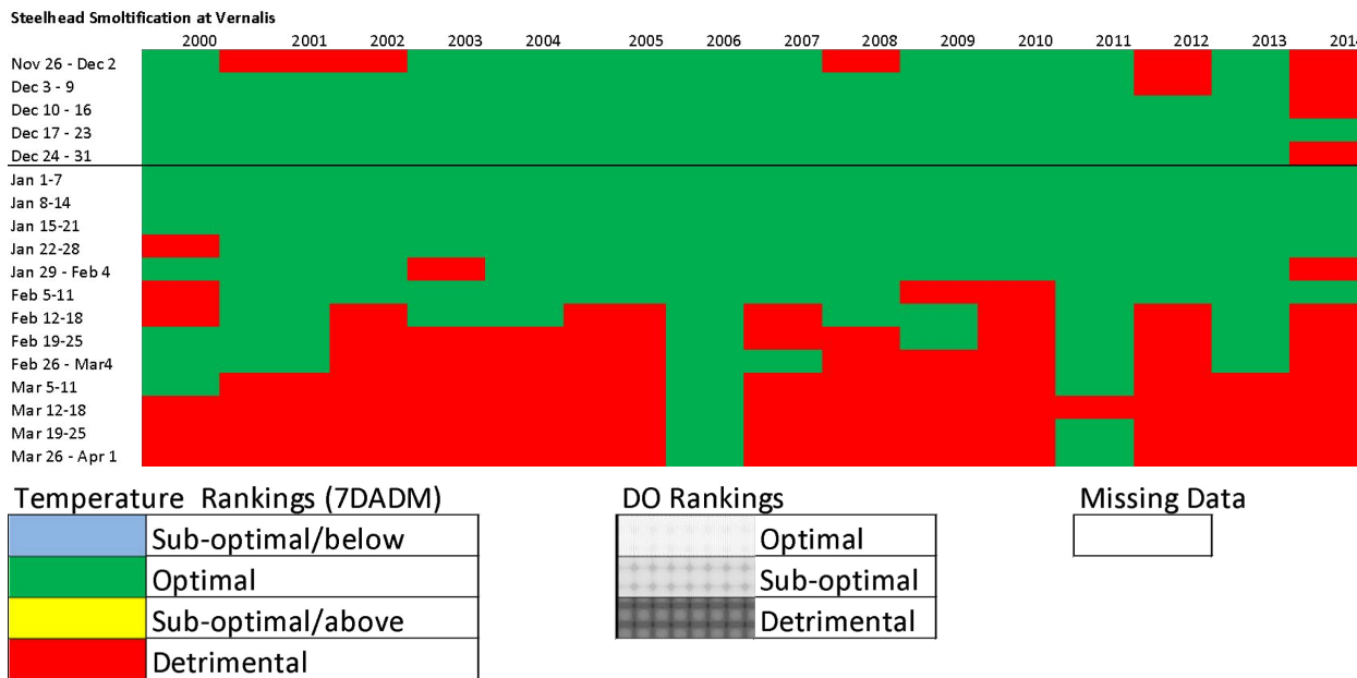
Figure 21 Steelhead Smoltification
