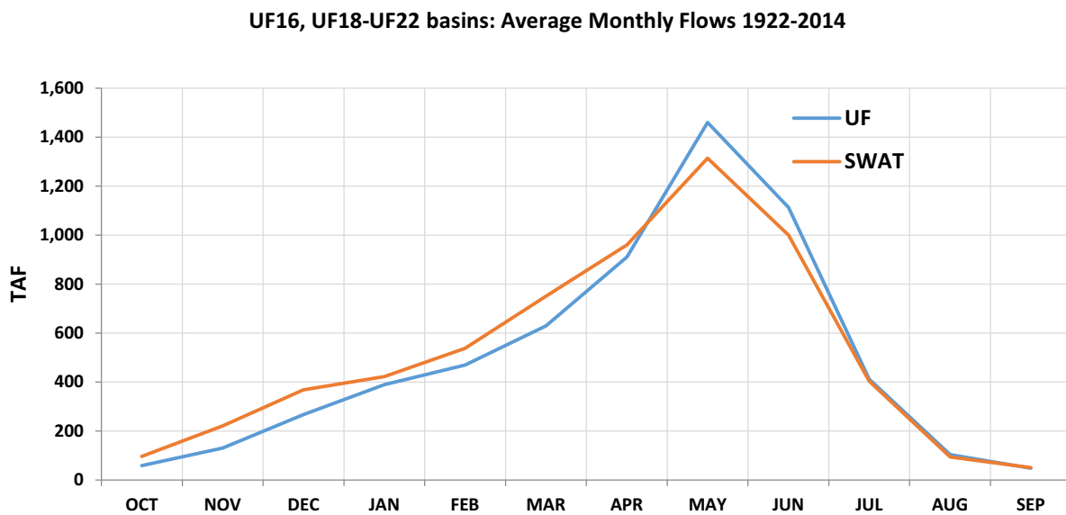
Figure 4-5. San Joaquin Valley SWAT Simulated Rim Inflows and Corresponding Unimpaired Estimated Flows
