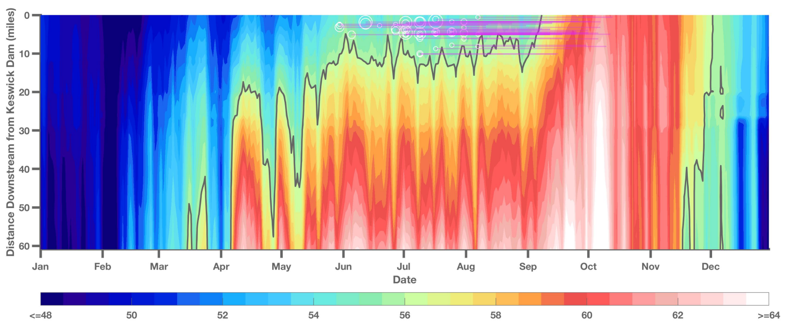
Daily Average Temperature (°F) Hindcast for Year 2014
