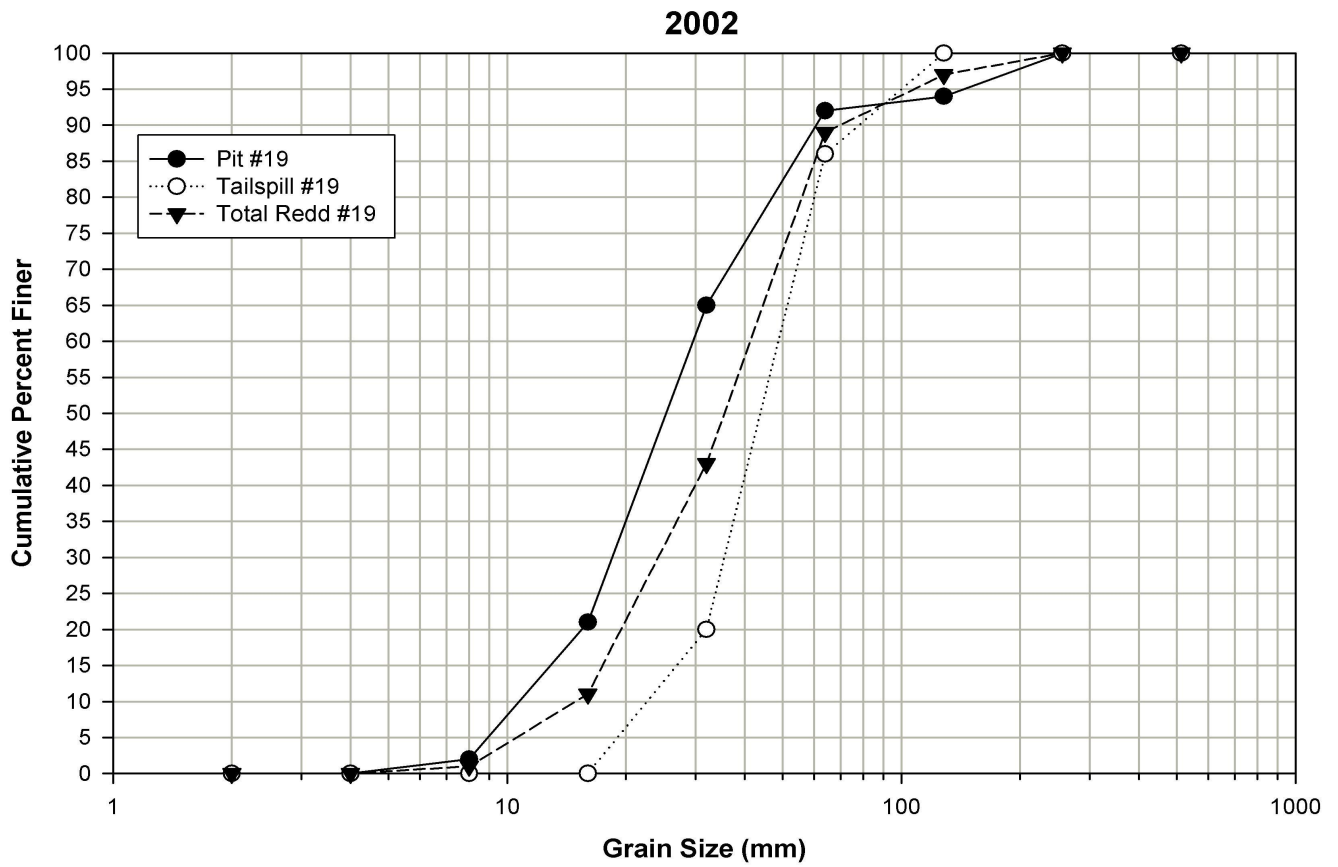
FIGURE A19.—Cumulative particle size distribution for Pebble Count No. 19 (Tables A6 and A7) performed in a spring Chinook redd on Clear Creek in 2002.
