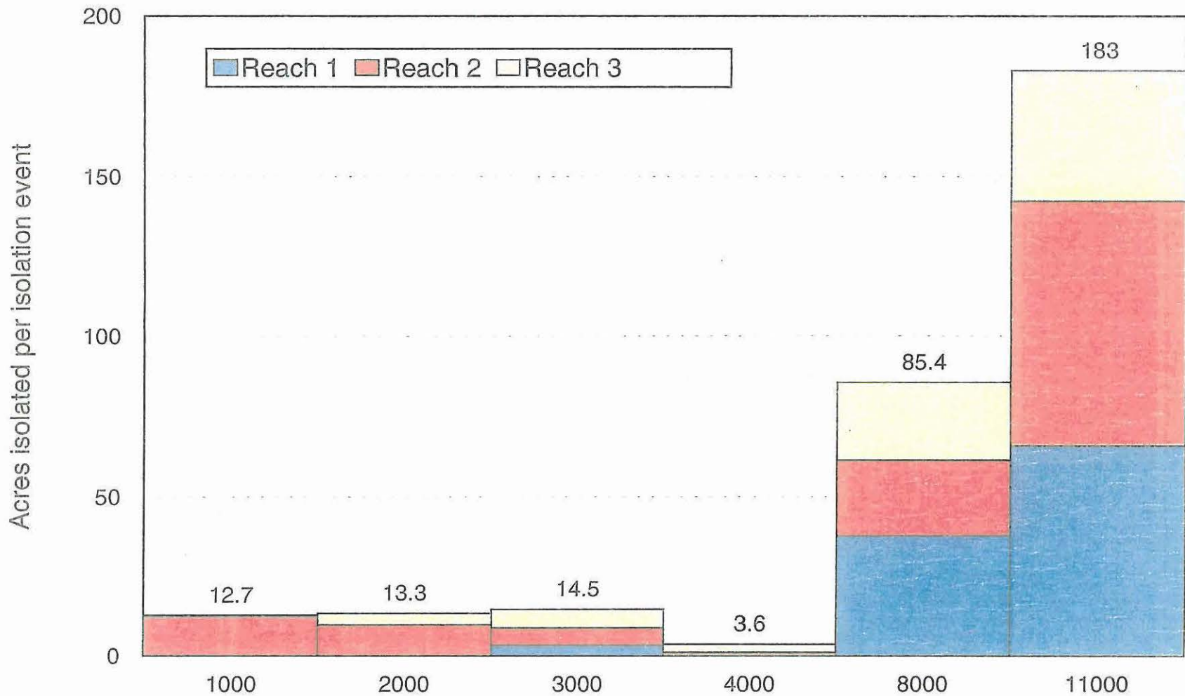
Figure 1. Total average of isolated areas relative to flow associated with isolation event measured during the lower American River flow fluctuation study, 1997 - 2000.
