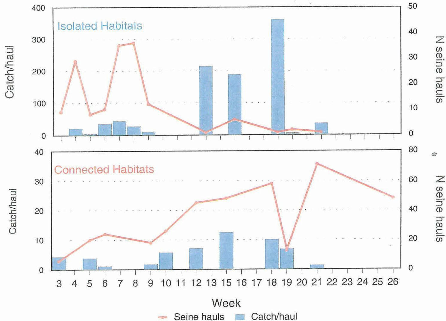
Figure 20. Effort (seine hauls) and catch-per-haul for chinook salmon collected during the lower American River flow fluctuation study, 1 January - 27 June 1997.
