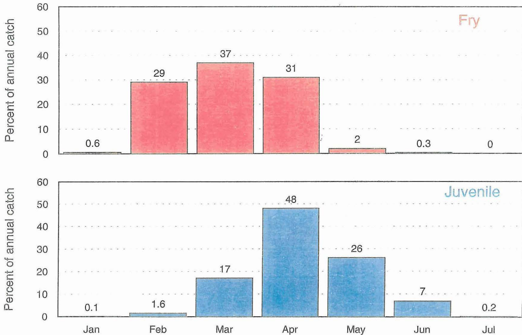
Figure 9. Mean monthly distribution of chinook salmon life stages observed during seining surveys on the lower American River, 1992 - 1995.
