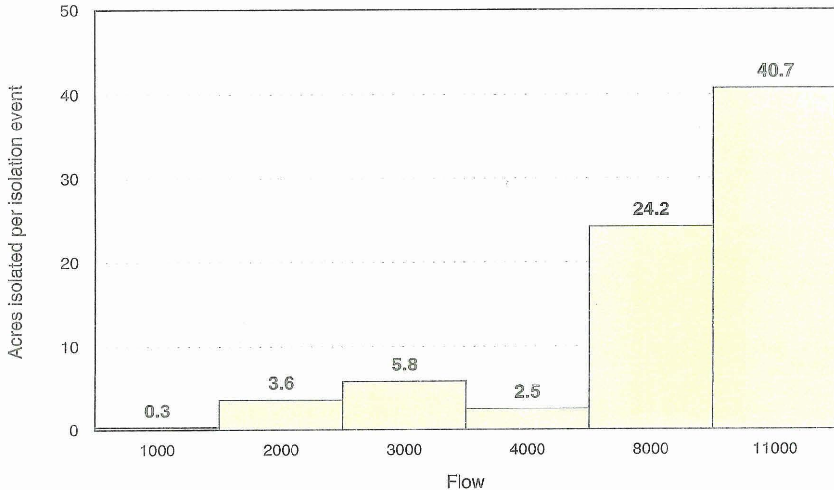
Figure 4. Total acreage of isolated areas in Reach 3 ( Ancil Hoffman Park to Nimbus Hatchery) relative to flow associated with isolation event measured during the lower American River flow fluctuation study, 1997 - 2000.
