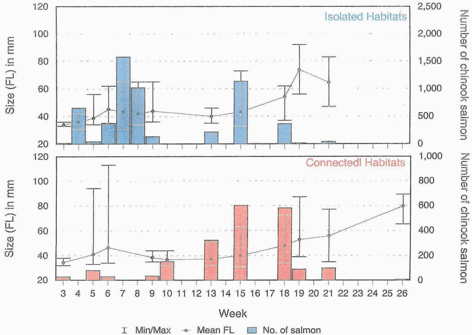
Figure 19. Total chinook salmon caught and the mean fork length (minimum and maximum) collected during the lower American River flow fluctuation study, 1 January - 27 June 1997.
