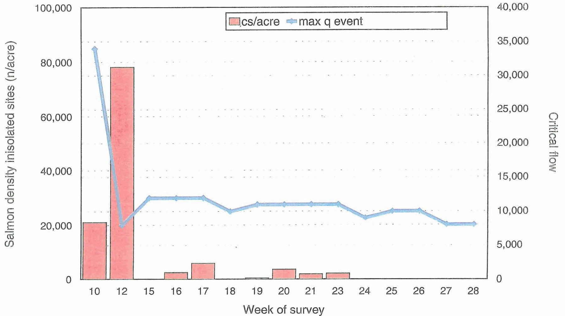
Figure 40. Salmon densities (n/acre) observed in isolated sites and critical flow preceding survey conducted in 1999 during the lower American River flow fluctuation investigation.
