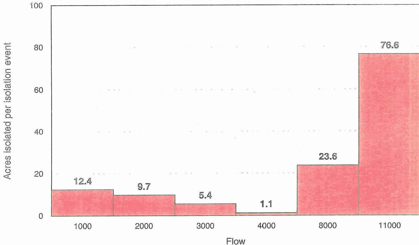
Figure 3. Total acreage of isolated areas in Reach 2 (Paradise Beach to Ancil Hoffman Park) relative to flow associated with isolation event measured during the lower American River flow fluctuation study, 1997 - 2000.
