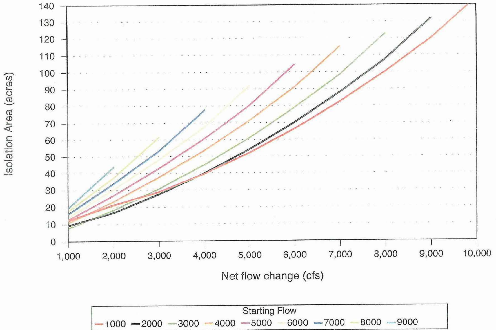
Figure 37. Incremental change in area of isolation associated with net change in flow for flows ranging from 1,000 to 10,000 cfs in the lower American River.
