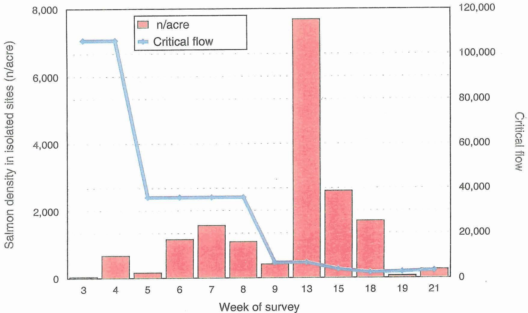
Figure 38. Salmon densities (n/acre) observed in isolated sites and critical flow preceding survey conducted in 1998 during the lower American River flow fluctuation investigation.
