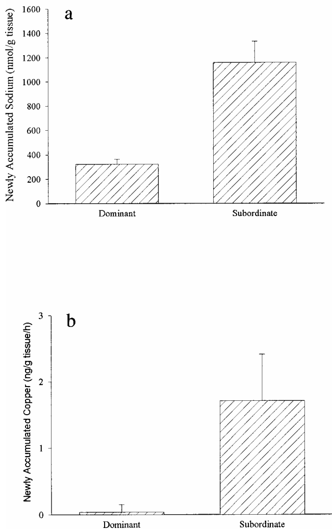
Fig. 2. Uptake of (a) waterborne sodium (measured using ^{22}\text{Na} ) and (b) waterborne copper (measured using ^{64}\text{Cu} ) from a dual labeling experiment. Data are presented as mean \pm standard error of the mean (independent samples t test: for sodium, t = -4.624 , p < 0.001 ; for copper, t = -2.333 , p = 0.035 ; n = 8 ).
