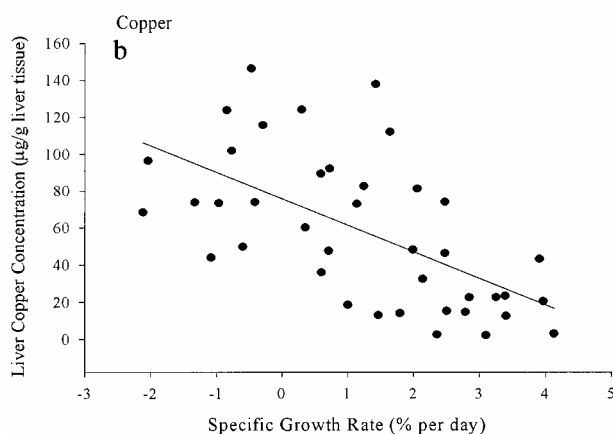
Fig. 6. (a) Liver copper concentrations for ranks of fish, where rank 1 is dominant, in the copper treatments (for each of ranks 1–4, n = 5 ; for each of ranks 5–10, n = 20 ). (b) Liver copper concentration was negatively correlated with specific growth rate for those fish in the experimental treatments (linear regression: F = 20.226 , r^2 = 0.364 , p < 0.001 ; n = 45 ).
