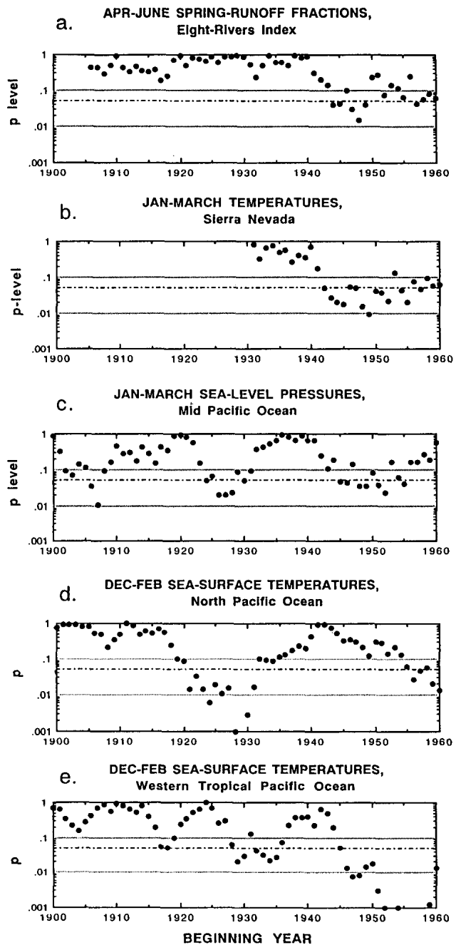
FIG. 4. Significance of trends in 30-yr moving windows of (a) eight rivers index spring runoff fraction, (b) a composite of winter-mean temperatures from central California, (c) winter-mean sea level pressures at 40^{\circ}\text{N} , 160^{\circ}\text{W} , (d) winter-mean sea surface temperatures between 35^{\circ}\text{--}50^{\circ}\text{N} and 180^{\circ}\text{--}150^{\circ}\text{W} , and (e) winter-mean sea surface temperatures between 10^{\circ}\text{S--}10^{\circ}\text{N} and 140^{\circ}\text{--}180^{\circ}\text{E} . Plotted are p levels for null hypothesis of stationary distribution using Kendall's tau statistic. Dot-dashed lines show p = 0.05 levels.
