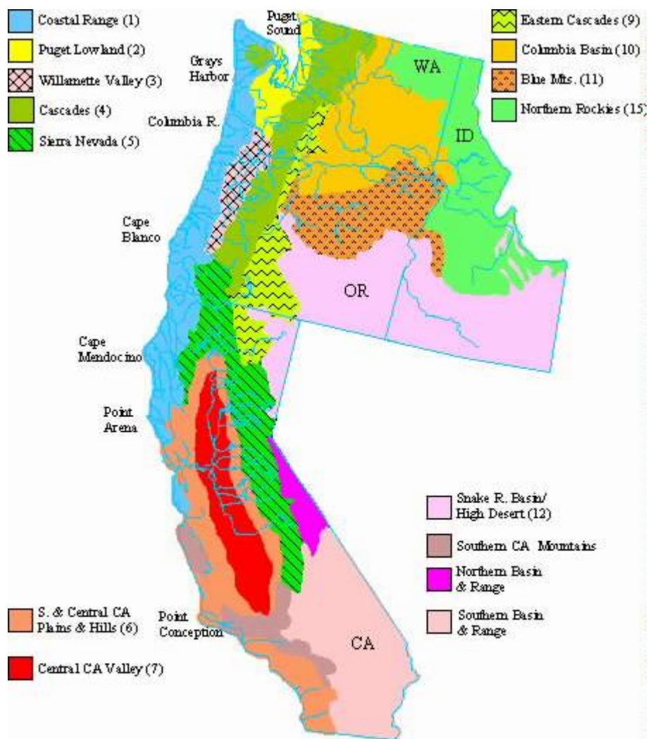
Figure 3. U.S. Environmental Protection Agency ecoregions for California, Idaho, Oregon, and Washington (Omernik and Gallant 1986, Omernik 1987). Regions are based on land use, climate, topography, potential natural vegetation, and soils. Ecoregions with number designations are described in the text.
