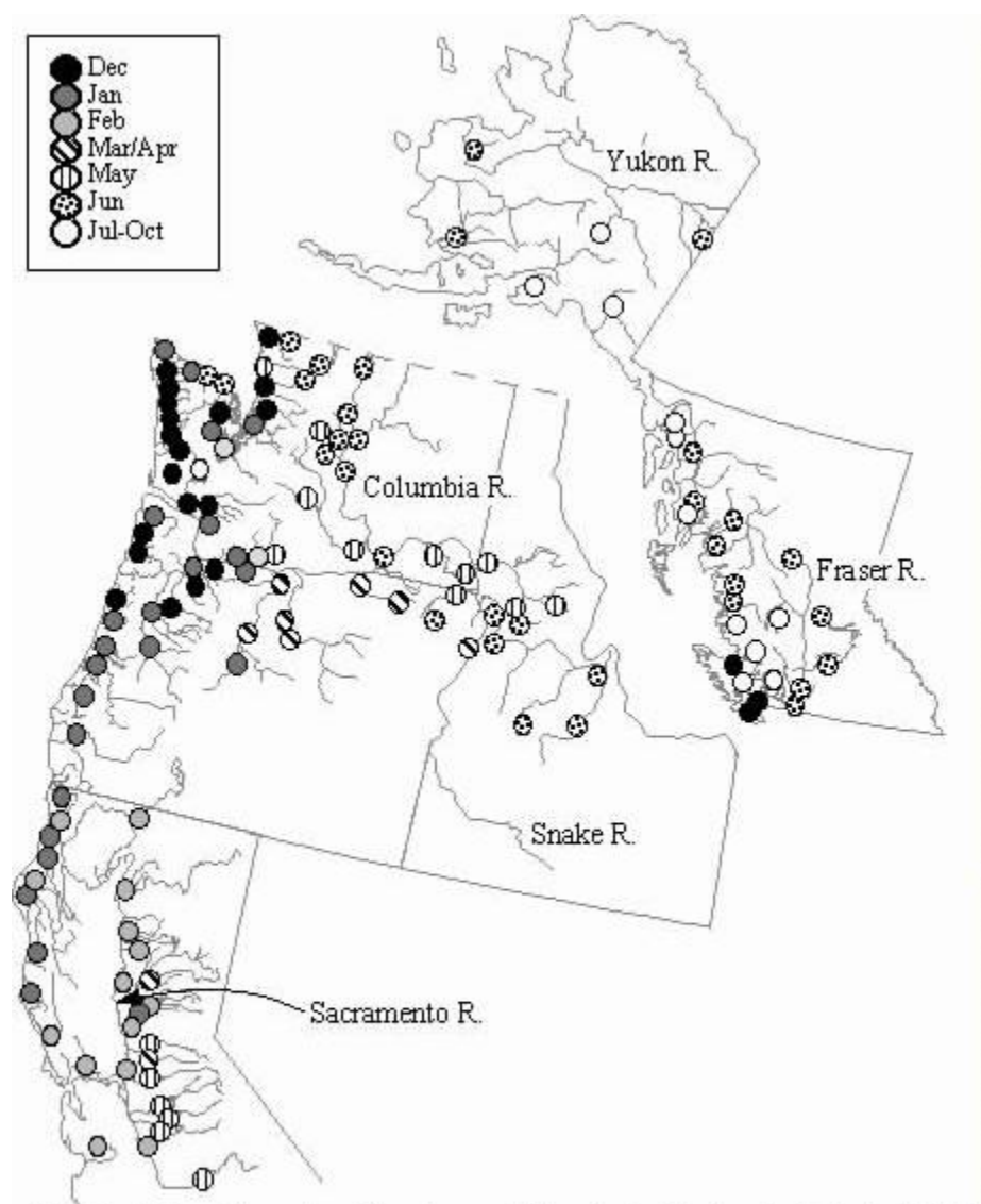
Figure 6. Timing of annual peak flow (by month) for selected river basins in Alaska, British Columbia, Washington, Oregon, California, and Idaho. If two peaks in flow occur, the higher of the two peaks is represented. Based on USGS streamflow data (Hydrosphere Data Products, Inc. 1993) and Inland Water Directorate streamflow data (Environment Canada 1991) (modified from Weitkamp et al. 1995).
