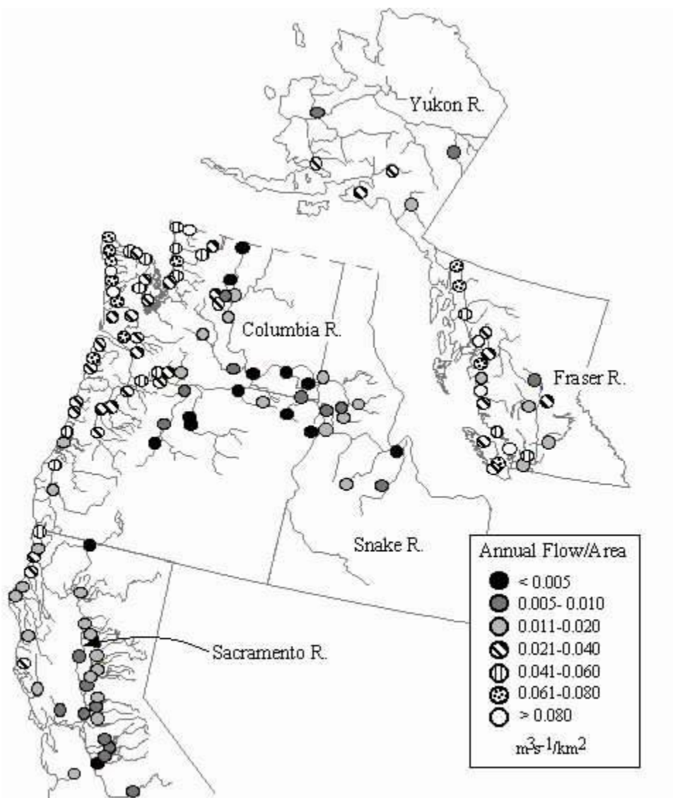
Figure 5. Average annual flow per area ( \text{m}^3\text{seconds}^{-1}\text{km}^{-2} ) for selected river basins in Alaska, British Columbia, Washington, Oregon, California, and Idaho. Values were calculated as the average annual flow for each gauging station divided by the reported gauged area. Based on USGS streamflow data (Hydrosphere Data Products, Inc. 1993) and Inland Water Directorate streamflow data (Environment Canada 1991) (modified from Weitkamp et al. 1995).
