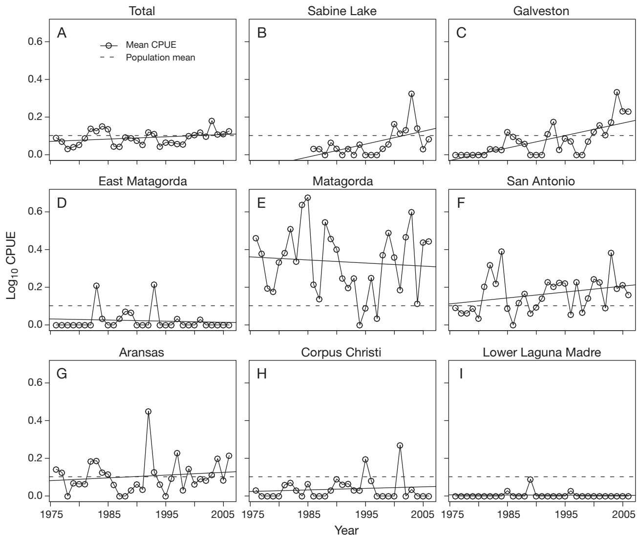
Fig. 2. Carcharhinus leucas . Young-of-the-year abundance in 8 estuarine embayments along the Texas coast (A: whole region; B to I: locations corresponding to Table 1). Inter-annual variation in \log_{10} catch per unit effort (CPUE; sharks \text{h}^{-1} ) within each site is evident (B to I; \circ = annual mean). Abundance in some sites fluctuates above and below the population mean (broken line), and therefore they vary in their suitability to meet the first criterion for a shark nursery (i.e. abundance in the area > mean abundance over all areas; Heupel et al. 2007). Portfolio effects may operate across these young-of-the-year habitats because variability in mean CPUE for the whole region (A) is less than the variability in individual sites. (From Froeschke et al. 2010b. With permission)
